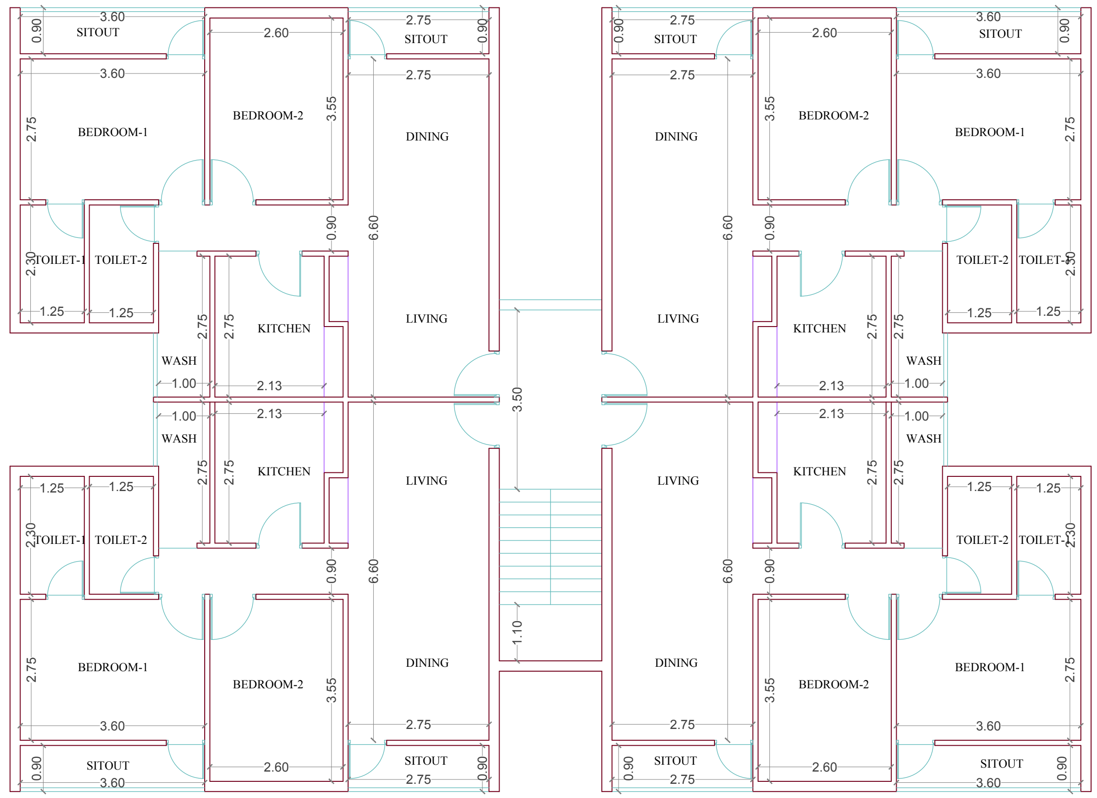
TYPICAL FLOOR
